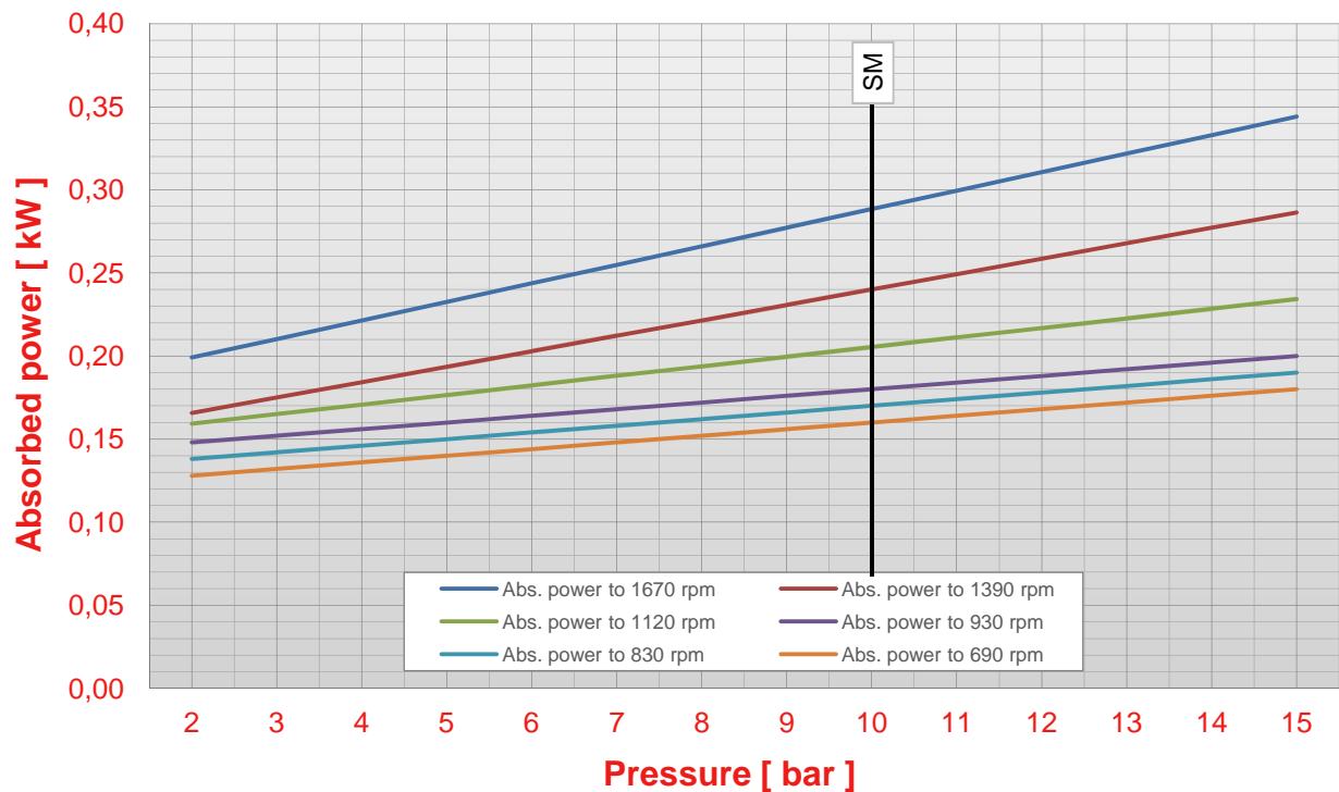
Pump S 05 pressure - abs. power chart (viscosity 50 cps)
