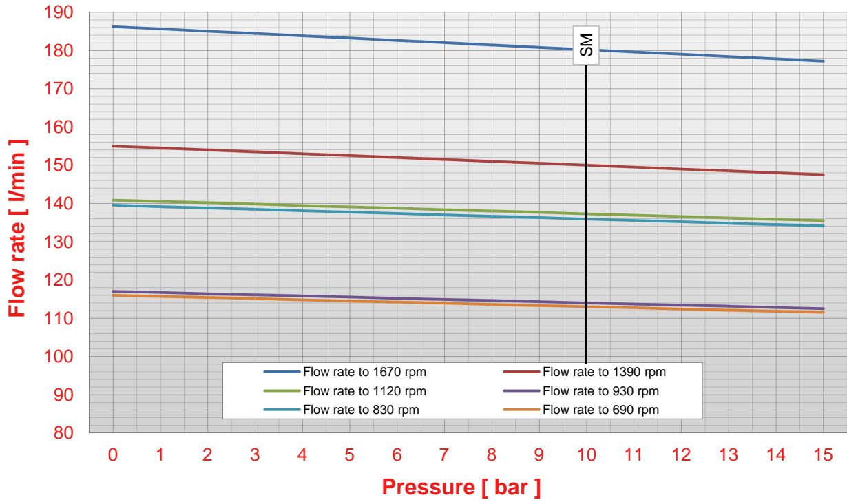
Pump S 150 pressure - flow rate chart (viscosity 50 cps)
