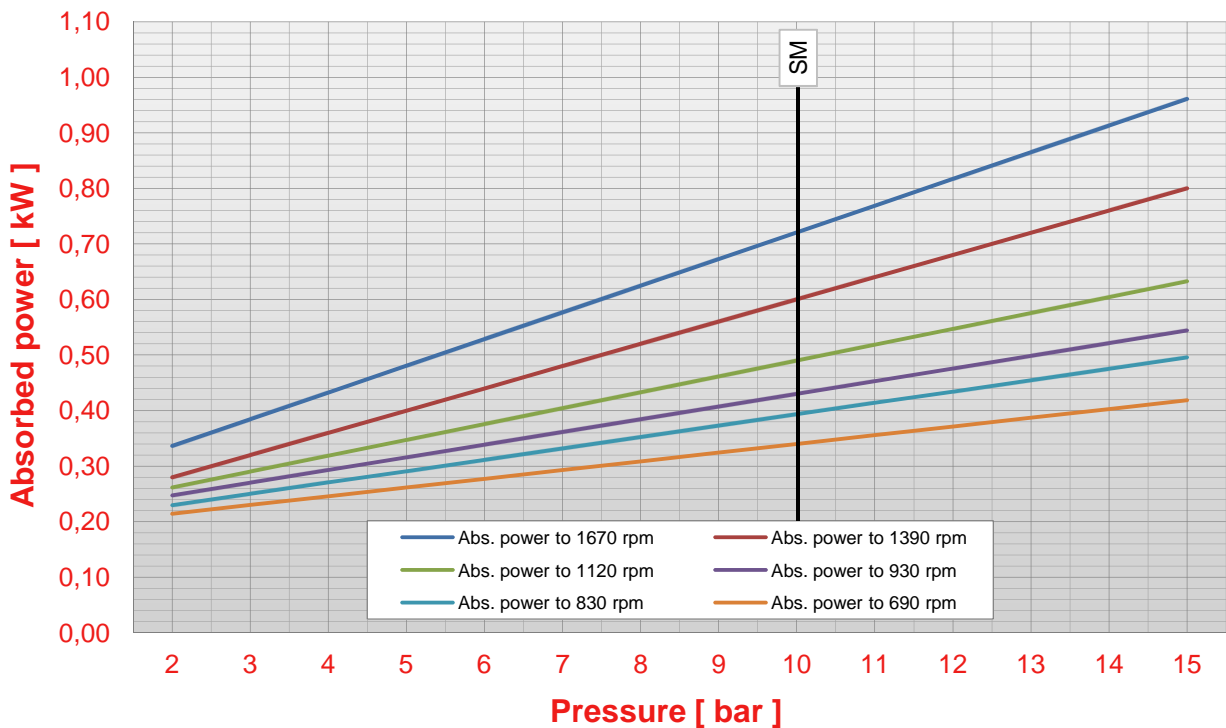
Pump S 25 pressure - abs. power chart (viscosity 50 cps)
