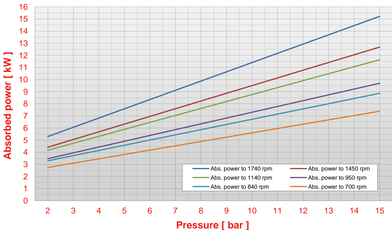
Pump S 400 pressure - abs. power chart (viscosity 50 cps)
