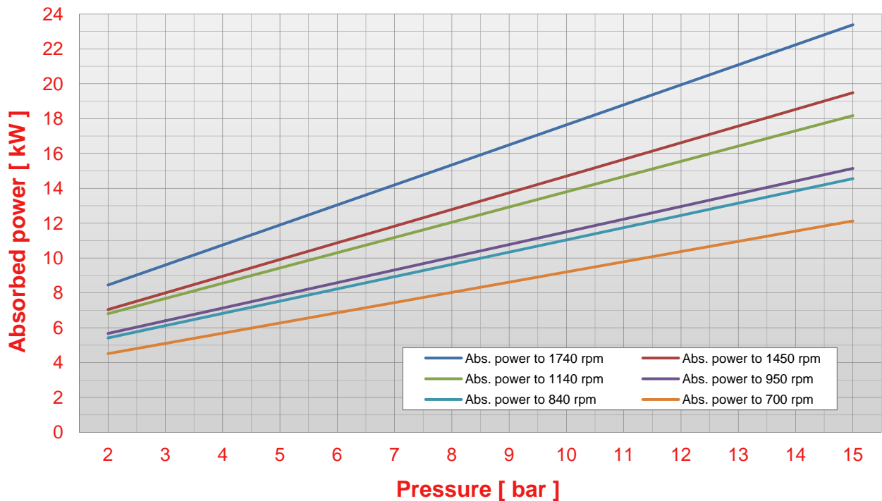
Pump S 600 pressure - abs. power chart (viscosity 50 cps)
