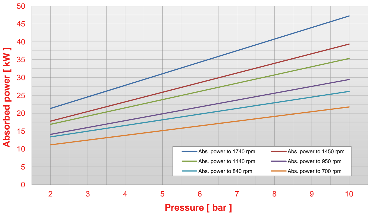
Pump N M60 pressure - abs. power chart (viscosity 50 cps)
