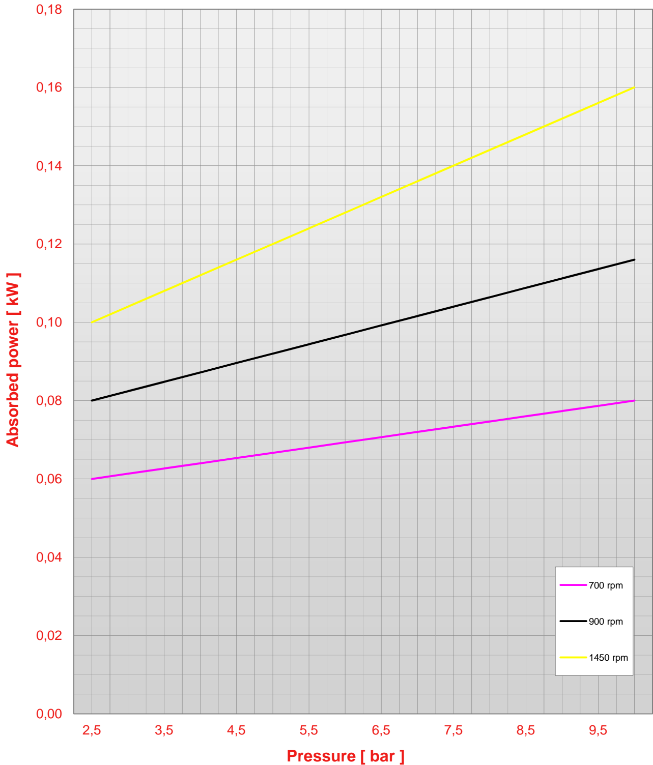
Pump WP 2 pressure - abs. power chart (viscosity 50 cps)
