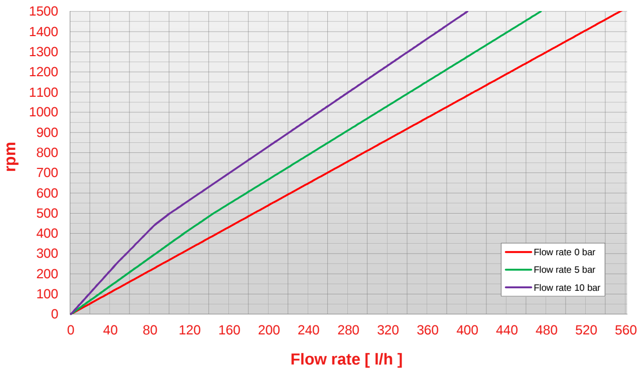
Pump WP 8 rpm - flow rate chart (viscosity 1 cps)
