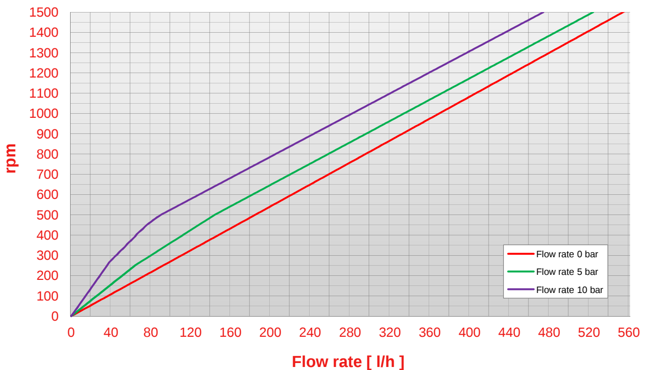
Pump WP 8 rpm - flow rate chart (viscosity 50 cps)
