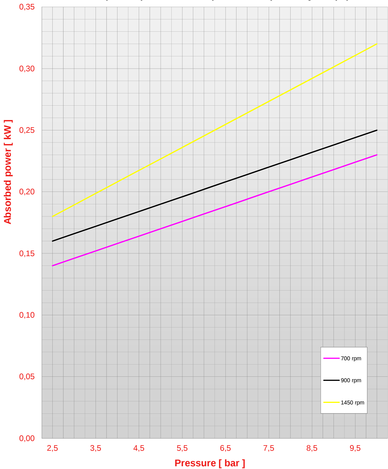
Pump WP 8 pressure - abs. power chart (viscosity 50 cps)
