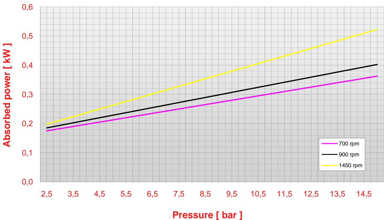
Pump N 10 pressure - abs. power chart (viscosity 50 cps)
