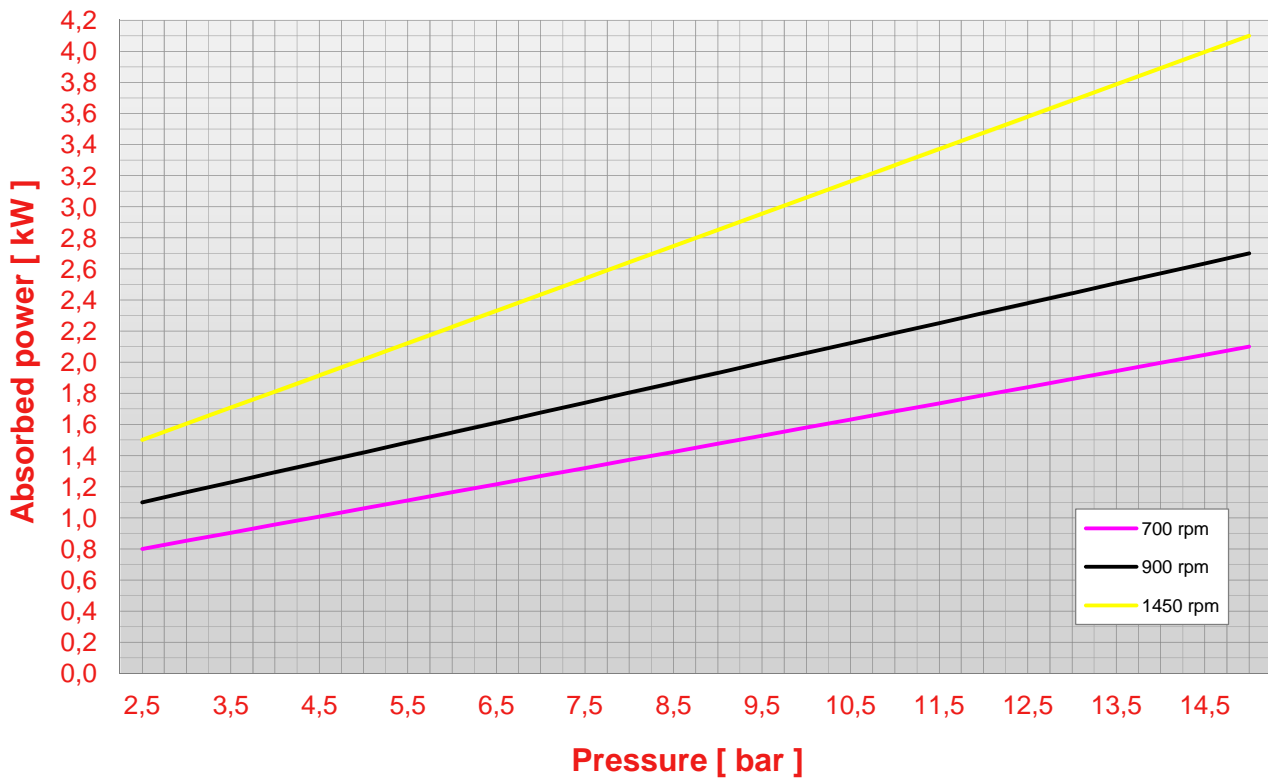
Pump N 100 pressure - abs. power chart (viscosity 50 cps)
