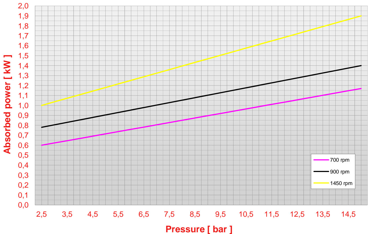
Pump N 136 pressure - abs. power chart (viscosity 50 cps)
