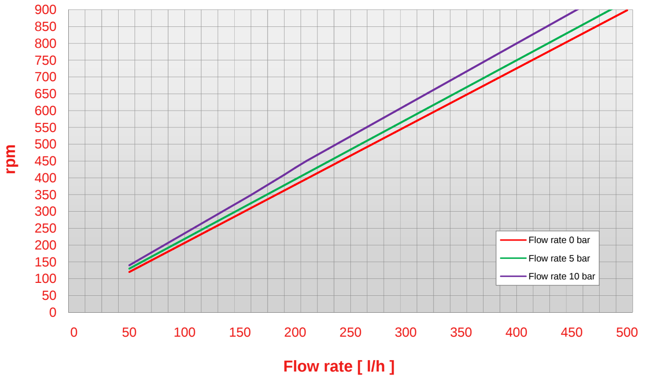
Pump N 14 rpm - flow rate chart (viscosity 1000 cps)
