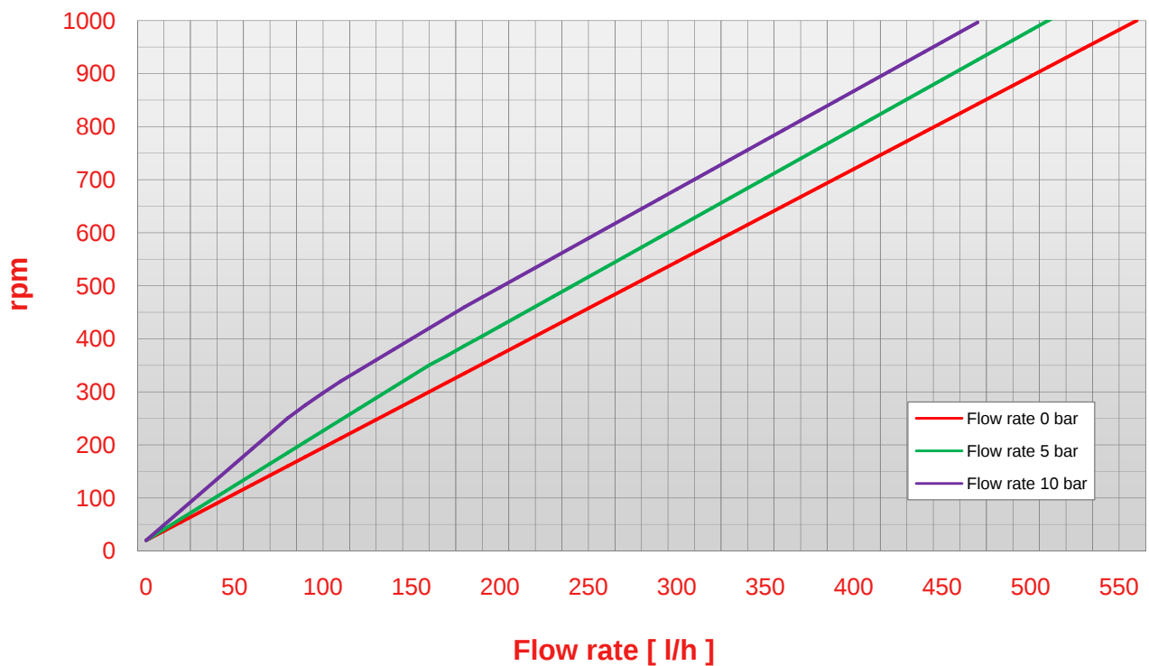
Pump N 14 rpm - flow rate chart (viscosity 100 cps)
