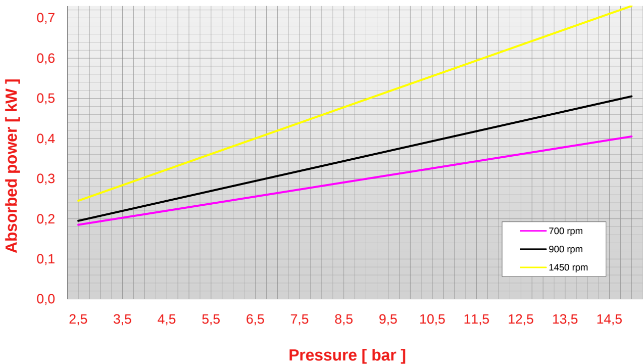
Pump N 14 pressure - abs. power chart (viscosity 50 cps)
