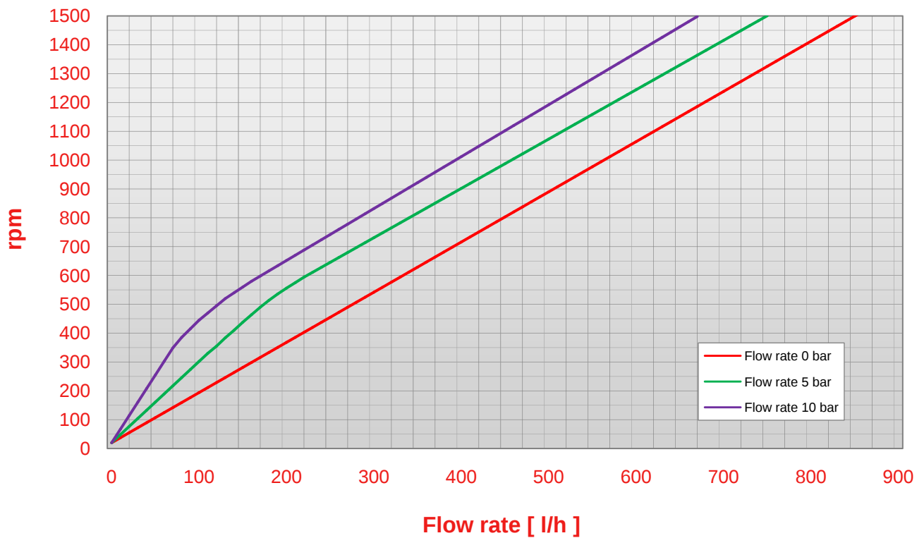
Pump N 14 rpm - flow rate chart (viscosity 1 cps)
