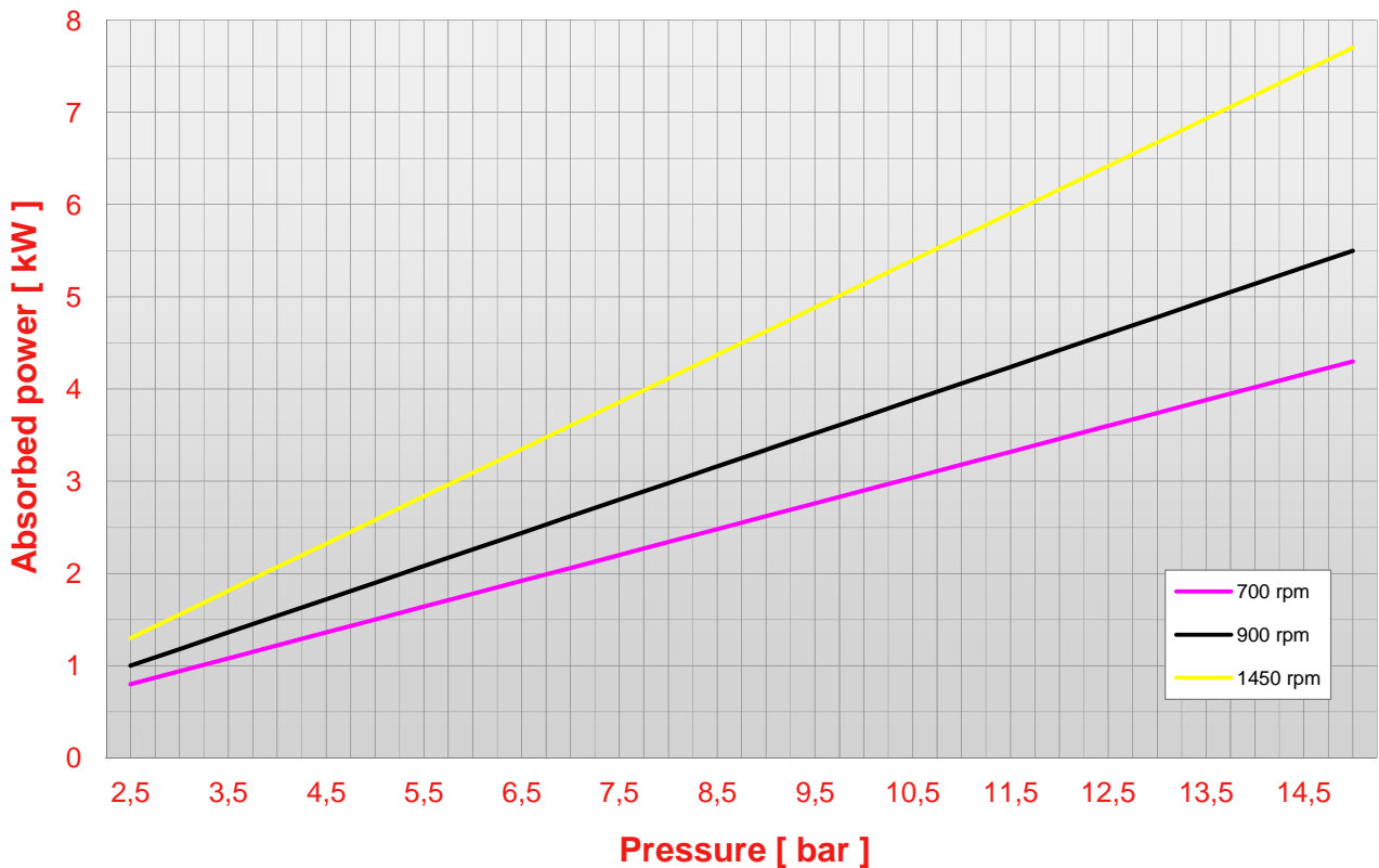
Pump N 200 pressure - abs. power chart (viscosity 50 cps)
