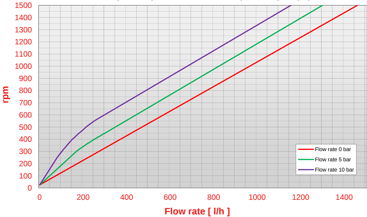
Pump N 24 rpm - flow rate chart (viscosity 1 cps)
