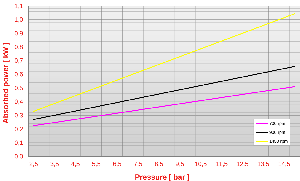
Pump N 24 pressure - abs. power chart (viscosity 50 cps)
