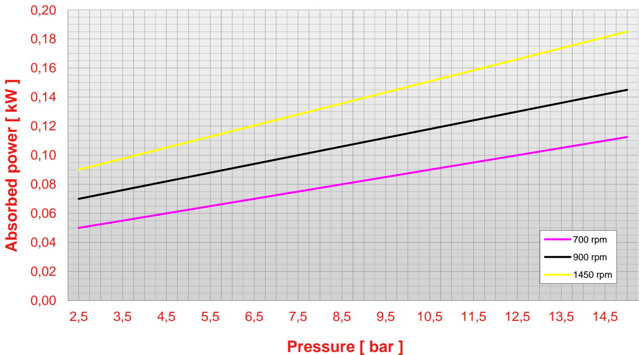
Pump N 2,5 pressure - abs. power chart (viscosity 50 cps)
