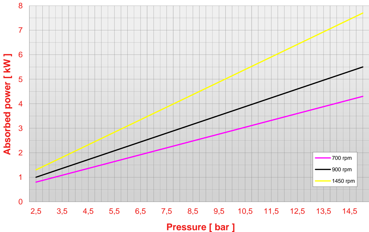
Pump N 300 pressure - abs. power chart (viscosity 50 cps)
