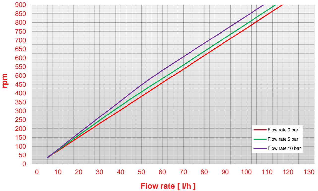
Pump N 3,5 rpm - flow rate chart (viscosity 500 cps)
