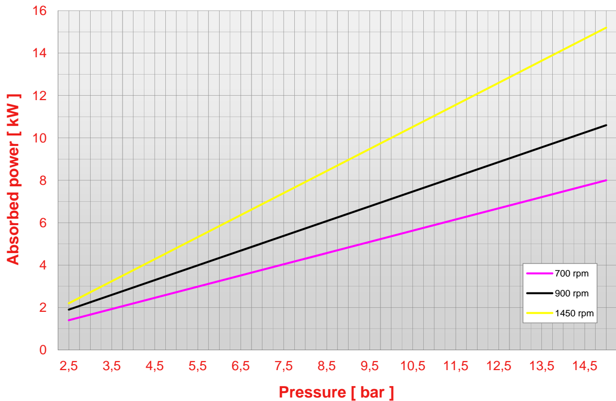
Pump N 400 pressure - abs. power chart (viscosity 50 cps)
