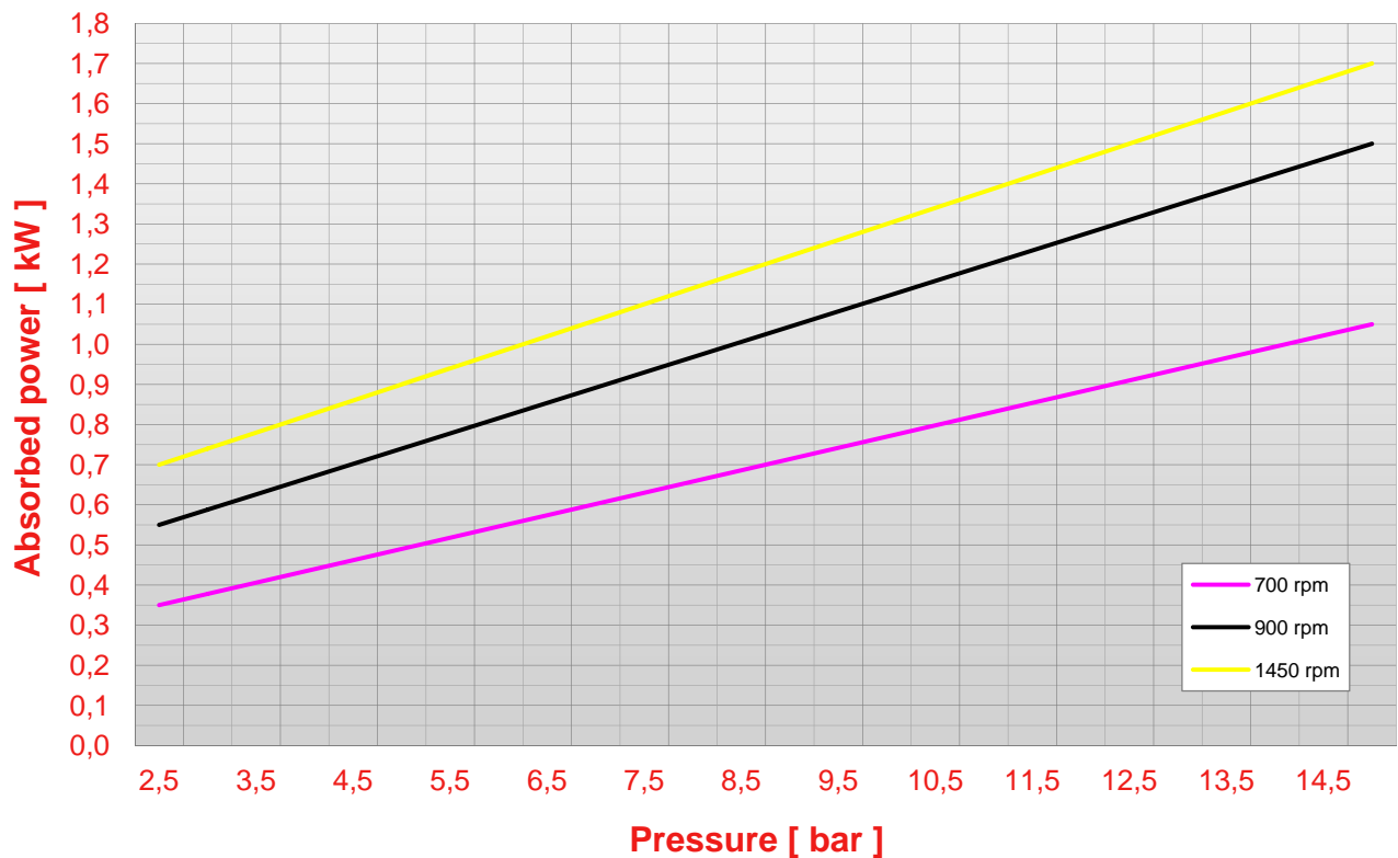
Pump N 41 pressure - abs. power chart (viscosity 50 cps)
