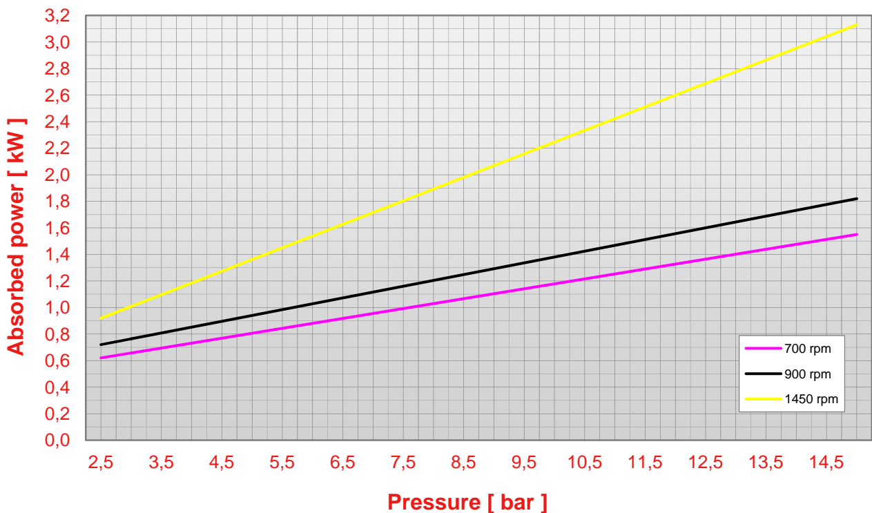
Pump N 68 pressure - abs. power chart (viscosity 50 cps)
