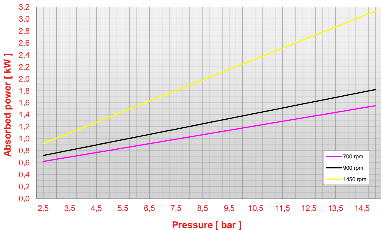
Pump N 68 pressure - abs. power chart (viscosity 50 cps)
