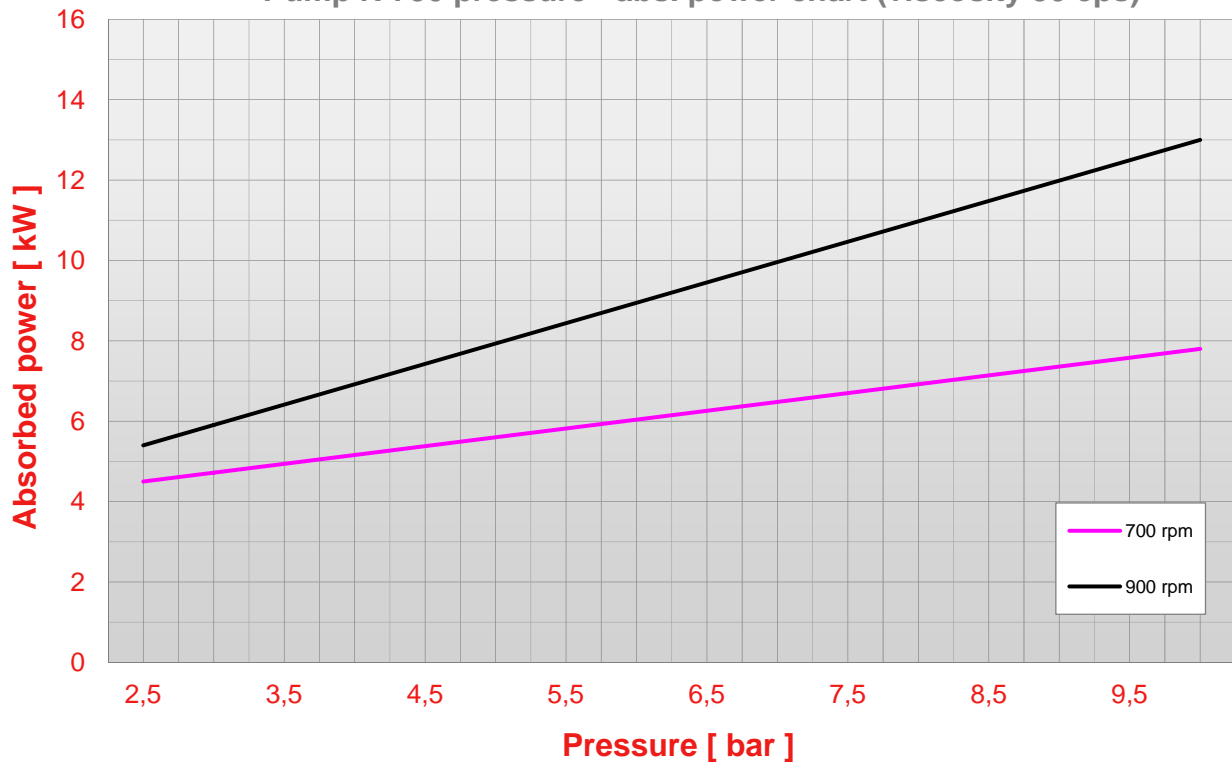
Pump N 750 pressure - abs. power chart (viscosity 50 cps)
