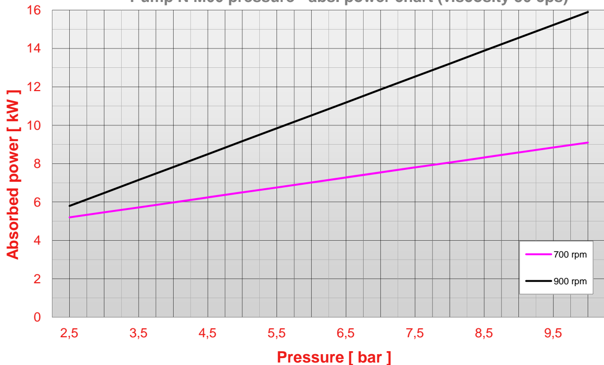
Pump N M00 pressure - abs. power chart (viscosity 50 cps)
